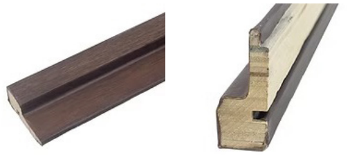
L-Shaped Trimer
